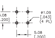
P.C. MOUNTING
