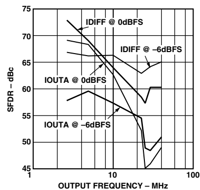
Figure 14. Differential vs. Single-Ended SFDR vs. f_{\text{OUT}} @ 100 MSPS
