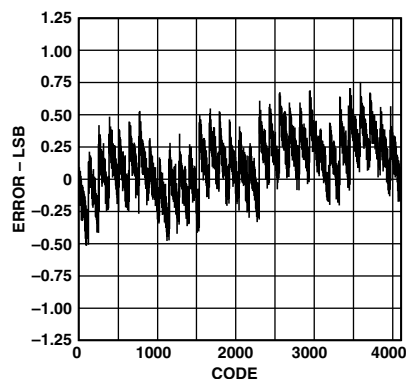
Figure 15. Typical INL
