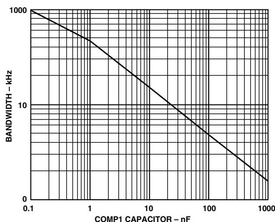
Figure 42. External COMP1 Capacitor vs. -3 dB Bandwidth
