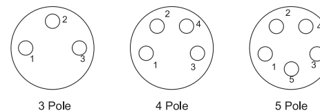
INSERT ARRANGEMENT
