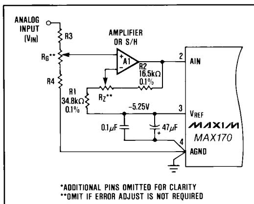
Figure 10. MAX170 Non-Inverting Bipolar Operation
