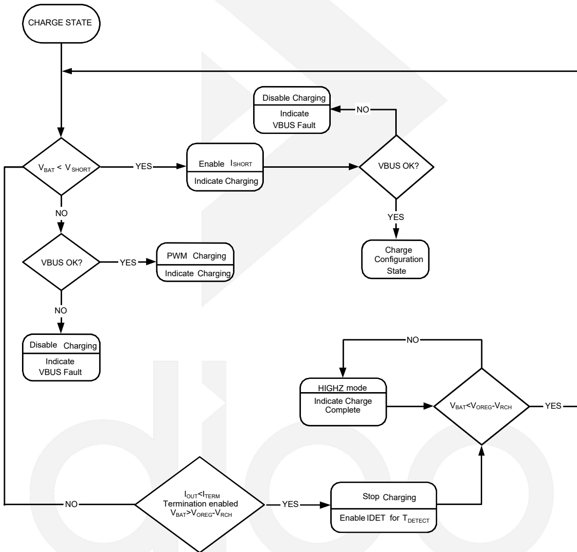
Figure 9. Charge Mode
