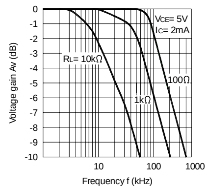
Fig.12 Frequency Response
