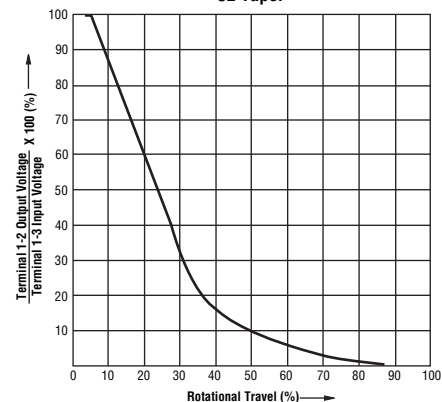
C2 Taper
