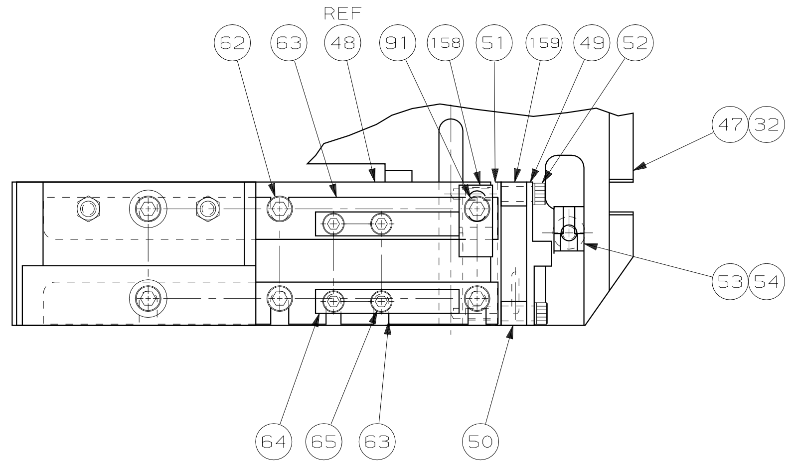
SECTION C-C
