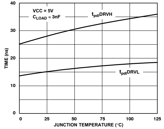
Figure 12. DRVH and DRVL t_{pd} vs. Temperature
