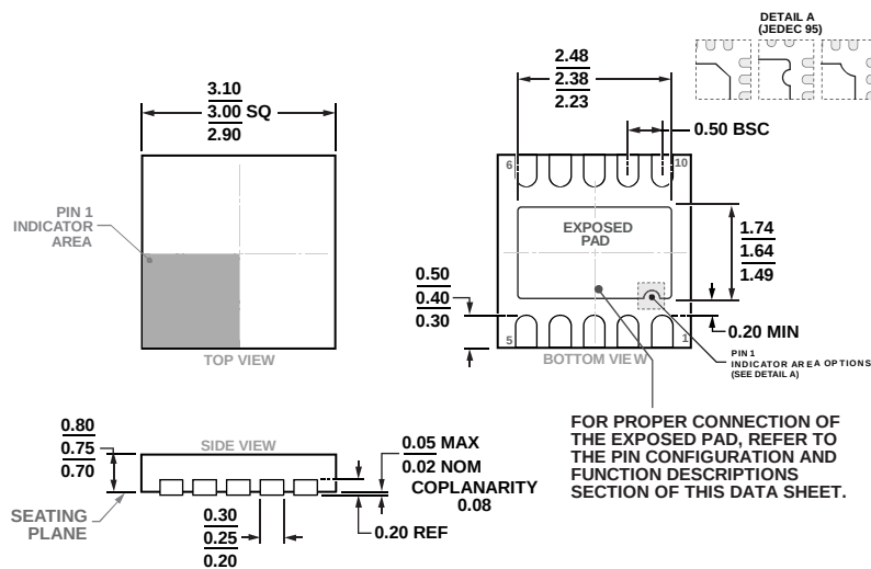
Figure 42. 10-Lead Lead Frame Chip Scale Package [LFCSF_WD] 3 mm × 3 mm Body, Very Very Thin, Dual Lead (CP-10-9) Dimensions shown in millimeters
