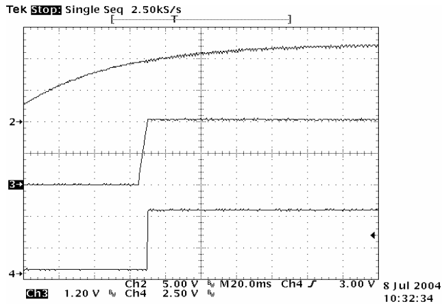
Figure 15: Turn on delay time at 12V in, 2.5V/20A out Ch2:Vin Ch3:Vout Ch4:PWRGD
