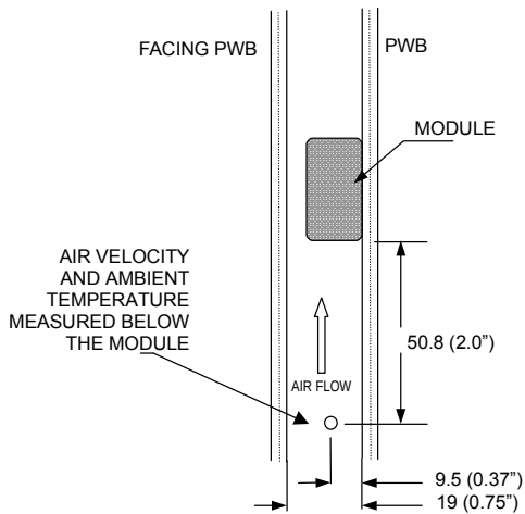
Figure 38: Wind tunnel test setup
