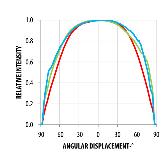
Figure 5: Radiation Pattern
