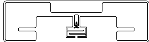
RF TAG 101.60X31.75 MM CASE 888AD/AE
