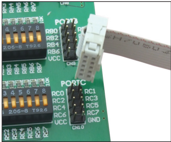
Figure 2: Plugging IDC10 connector into a development system
