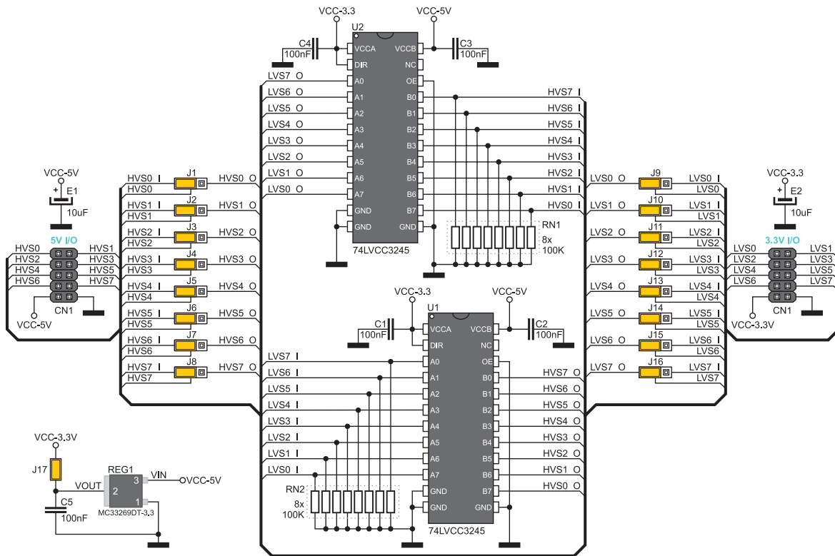
Figure 9: Additional board connection schematic
