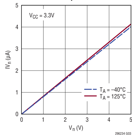
V_n Input Current vs Voltage: All Modes Except \pm ADJ
