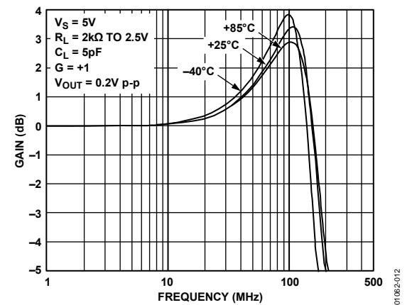
Figure 12. AD8054 Gain vs. Frequency vs. Temperature
