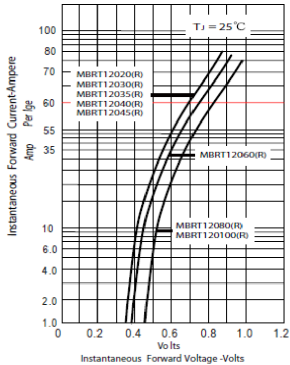
Figure.1-Typical Forward Characteristics
