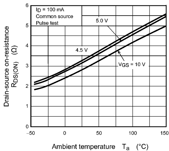
Fig. 7.5 R_{DS(ON)} - T_a
