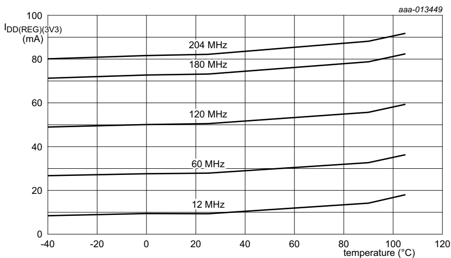
Fig 11. Typical supply current versus temperature in active mode
