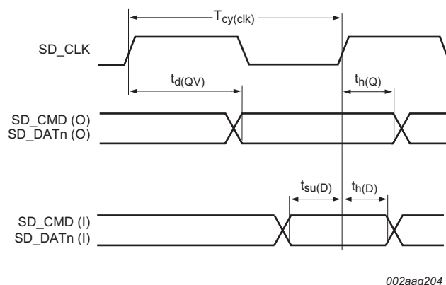
Fig 39. SD/MMC timing
