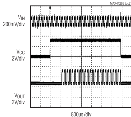
POWER-UP RESPONSE
