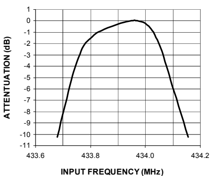
Bandpass Filter Attenuation f_{XTAL} = 13.52313MHz
