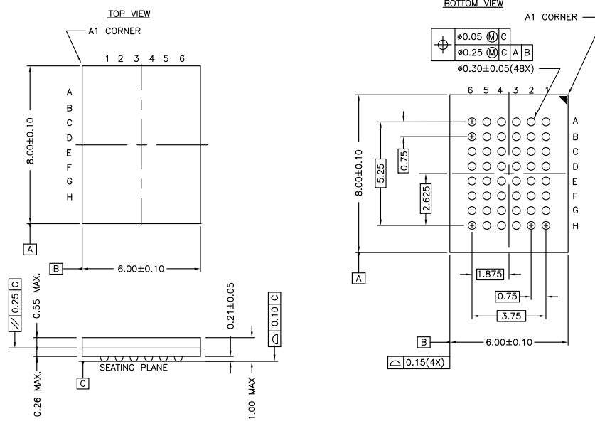
Figure 12. 48-ball VFBGA ( 6 \times 8 \times 1.0 mm) BV48/BZ48 Package Outline, 51-85150
