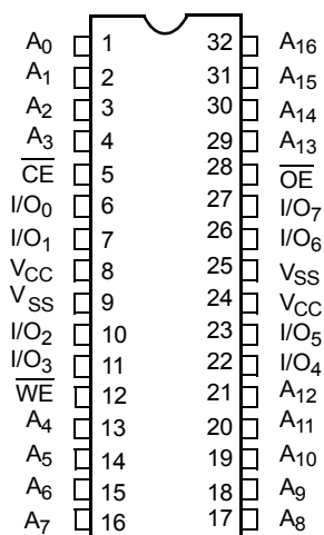
Figure 2. 32-pin SOJ / TSOP II (Top View)
