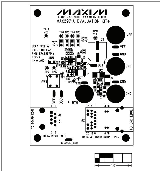
Figure 2. MAX5971A EV Kit Component Placement Guide— Component Side
