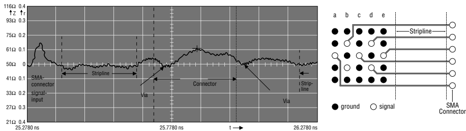
TDR plot showing the impedance progression from a 2mm H.M. connector. Signal ground pattern as shown.
