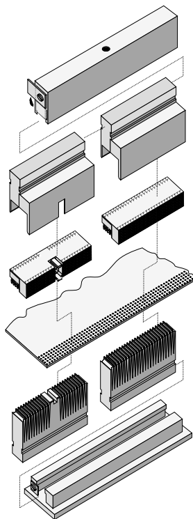
Modular press-fit tool for female connector modules 5+2
