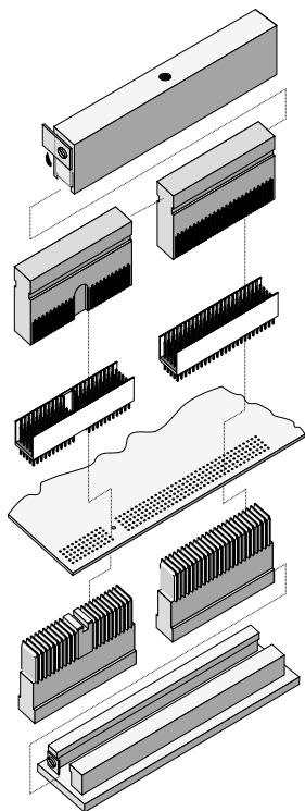
Modular press-fit tool male connector modules 5+2
