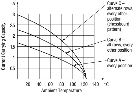
Current Rating For Various Contact Mounting Configurations
