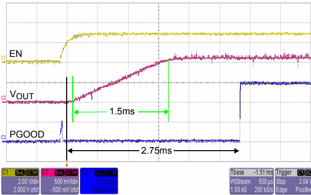
FIGURE 1. SOFT-START SEQUENCE
