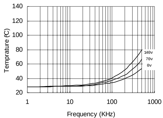
Figure 22. IR2183 vs. Frequency (IRFBC20), R_{gate} = 33\Omega , V_{CC} = 15V
