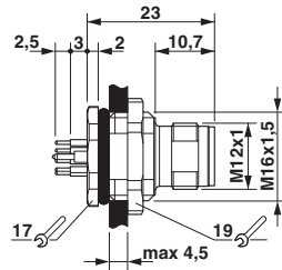
Dimensioned drawing
