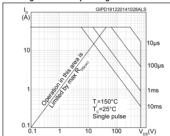
Figure 4. Safe operating area for IPAK
