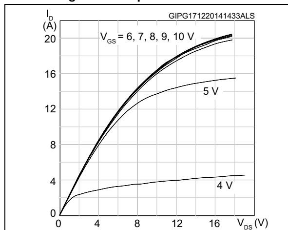
Figure 6. Output characteristics
