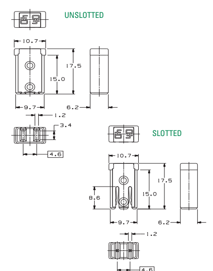
Dimensions MCASE+®
