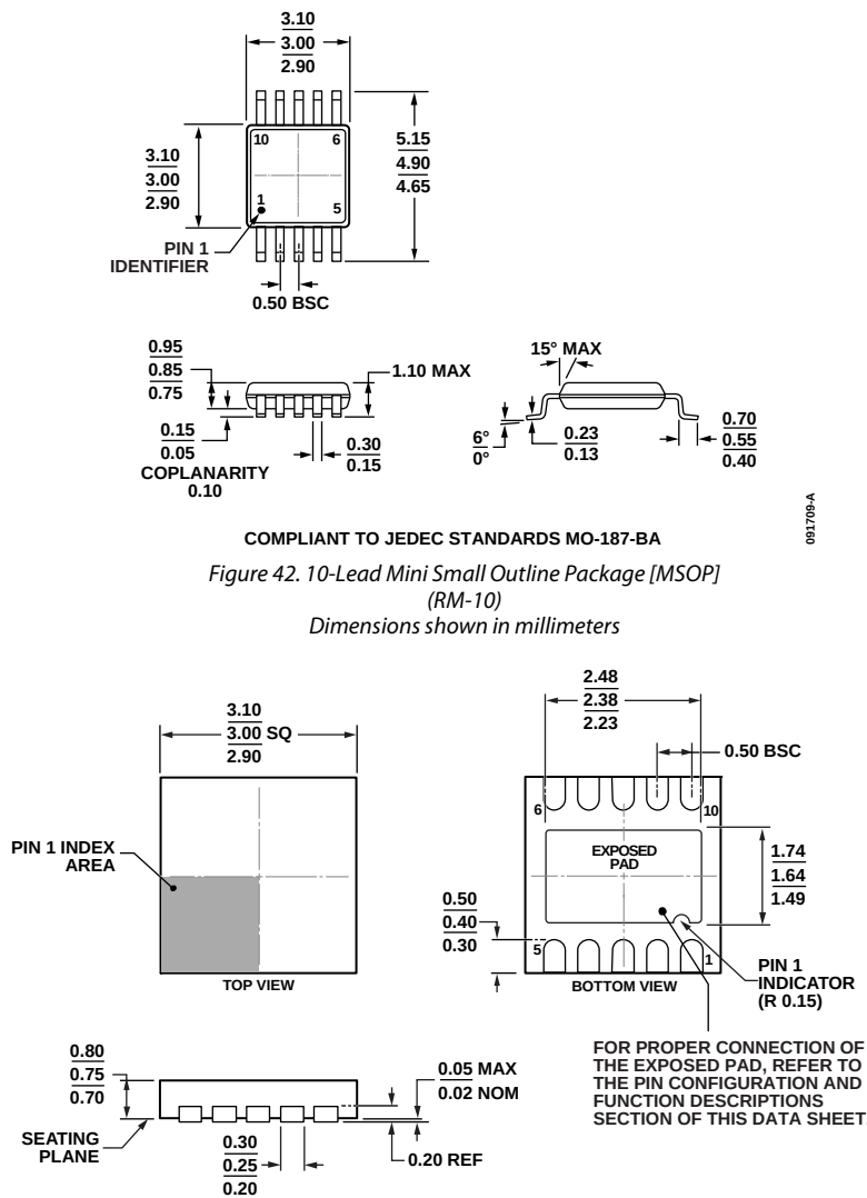
Figure 43. 10-Lead Lead Frame Chip Scale Package [QFN (LFCSP_WD)] 3 mm × 3 mm Body, Very Very Thin, Dual Lead (CP-10-9) Dimensions shown in millimeters
