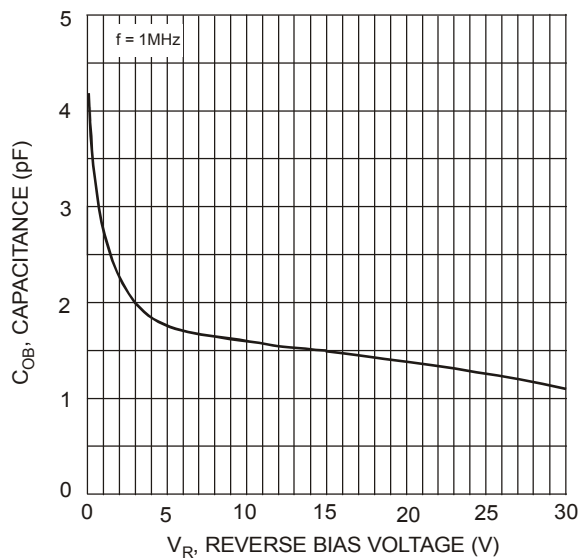
Fig. 4 Output Capacitance
