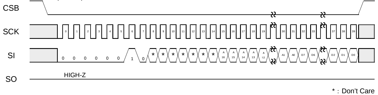
Figure 40. Write command
