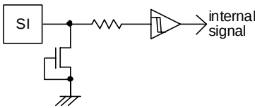
Figure 55. SI input equivalent circuit
