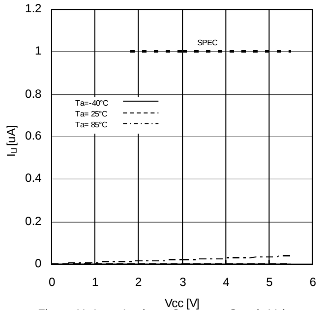
Figure 11. Input Leakage Current vs Supply Voltage (CSB,SCK,SI,HOLDB,WPB)
