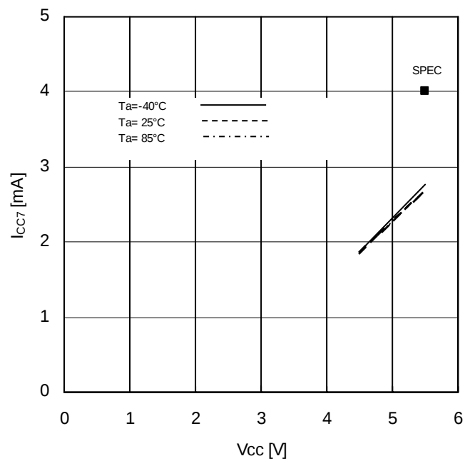
Figure 18. Supply Current (Read) vs Supply Voltage (fSCK=10MHz)
