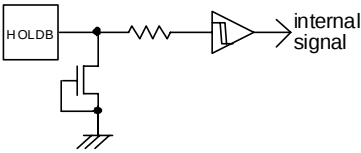
Figure 56. HOLDB input equivalent circuit
