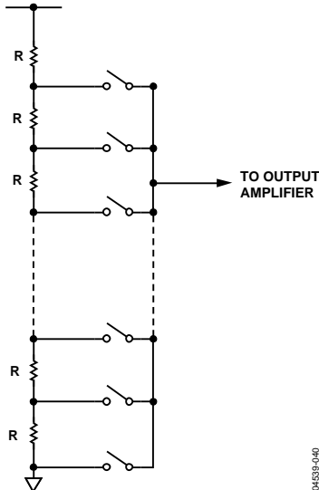
Figure 39. Resistor String
