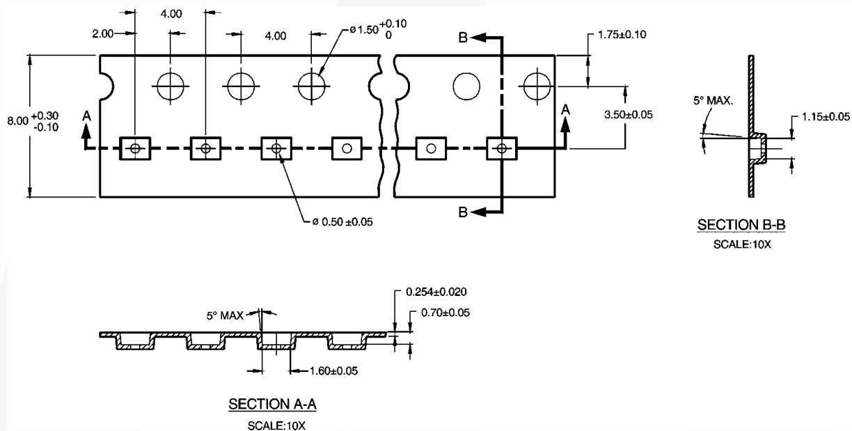
Tape Dimension inches (millimeters)
