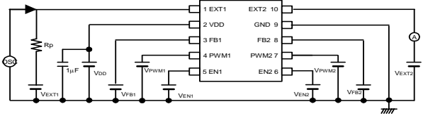
Circuit 7
