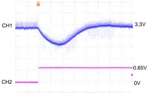
400µsec/div CH1:Vout2 , AC-COUPLED ,10mV/div CH2:PWM2 , 0.5V/div
