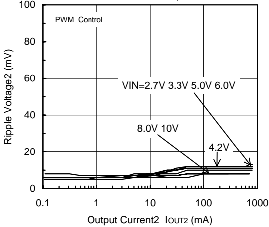
FOSC=300kHz, VOUT2=1.8V
