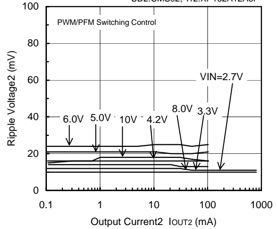
FOSC=300kHz, VOUT2=1.8V
