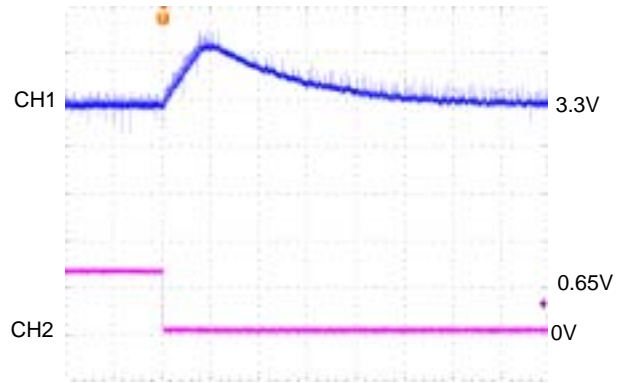
200μsec/div CH1:V out2 , AC-COUPLED ,20mV/div CH2:PWM2 , 0.5V/div
