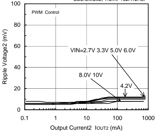
FOSC=300kHz, VOUT2=1.8V
