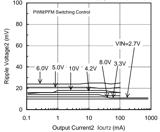
FOSC=300kHz, VOUT2=1.8V
