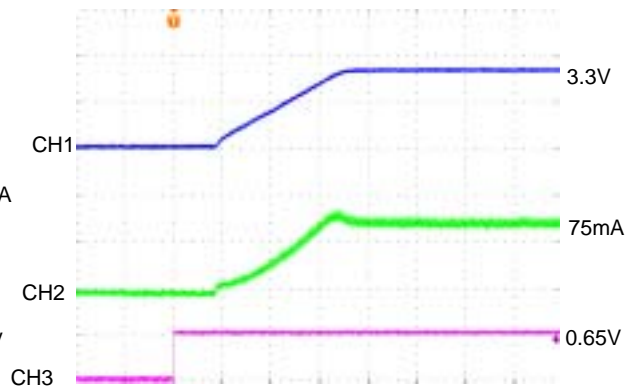
4ms/div CH1:V out2 , 2.0V/div CH2:I IN2 , 50mA/div CH3:EN2 , 0.5V/div
