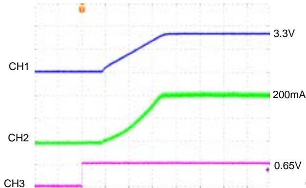
4ms/div CH1:V out2 , 2.0V/div CH2:I IN2 , 100mA/div CH3:EN2 , 0.5V/div
