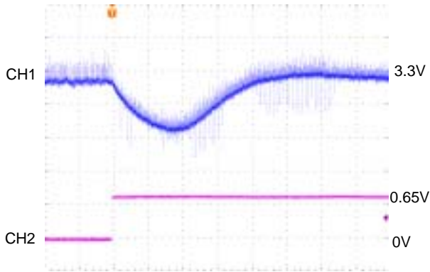
400μsec/div CH1:V out2 , AC-COUPLED ,10mV/div CH2:PWM2 , 0.5V/div
