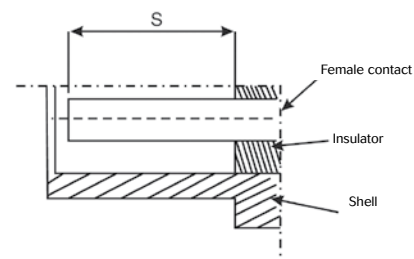
Female connector
