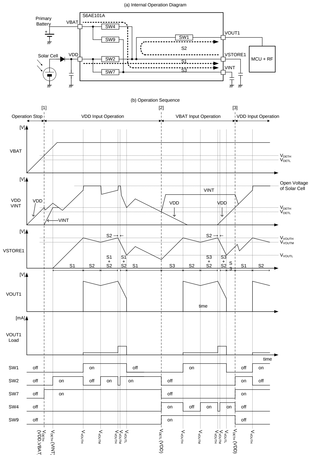
Figure 7-4 Input Power Switching
