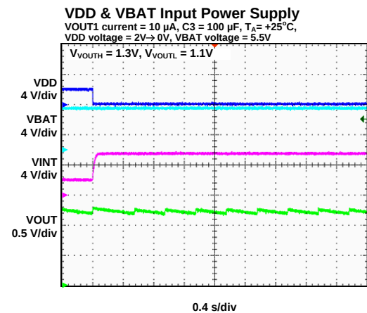
S6AE101AGraph030
