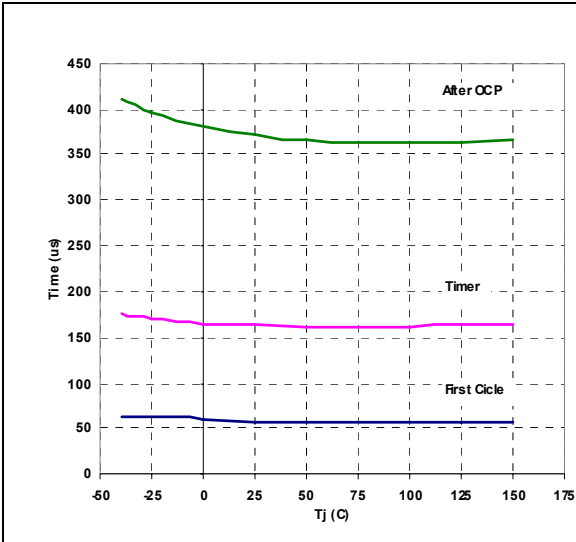
Figure 34. Start-up timer period vs T_J
