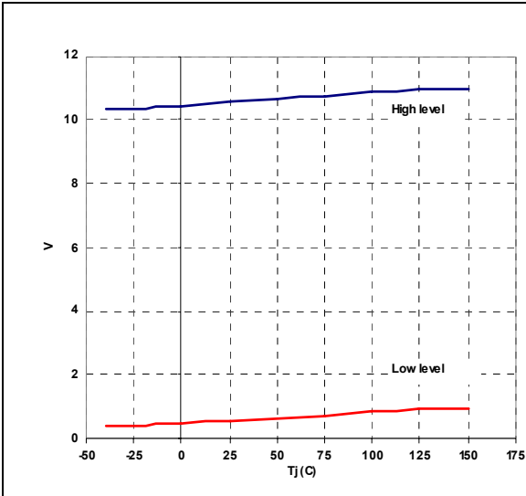
Figure 32. Gate drive output saturation vs T_J
