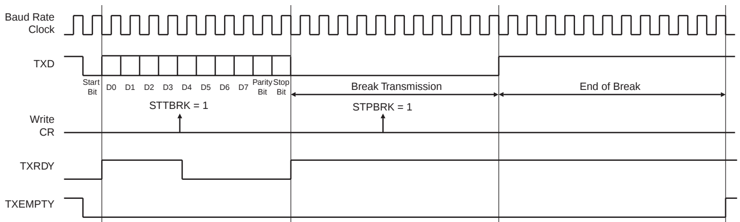
Figure 20-14. Break Transmission
