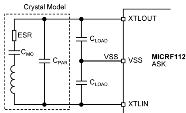
Figure 4. Reference Oscillator ASK Operation
