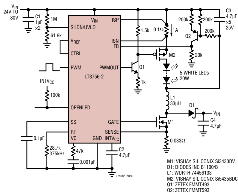
Buck Mode 1A LED Driver with High Dimming Ratio and Open LED Reporting
