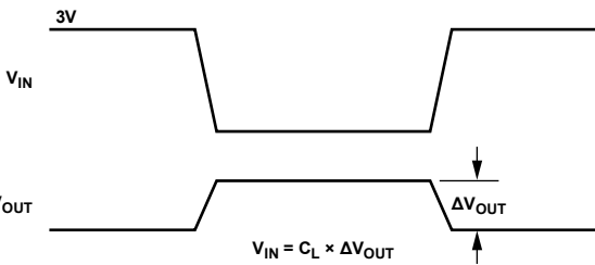
Figure 21. Charge Injection
