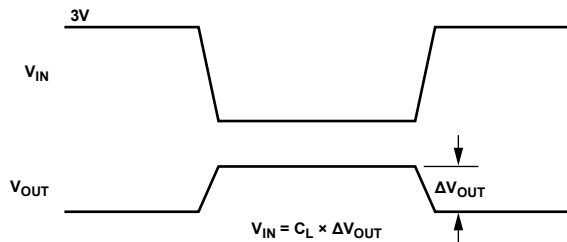
Figure 21. Charge Injection
