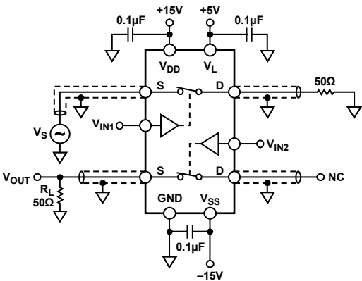
Figure 23. Channel-to-Channel Crosstalk
