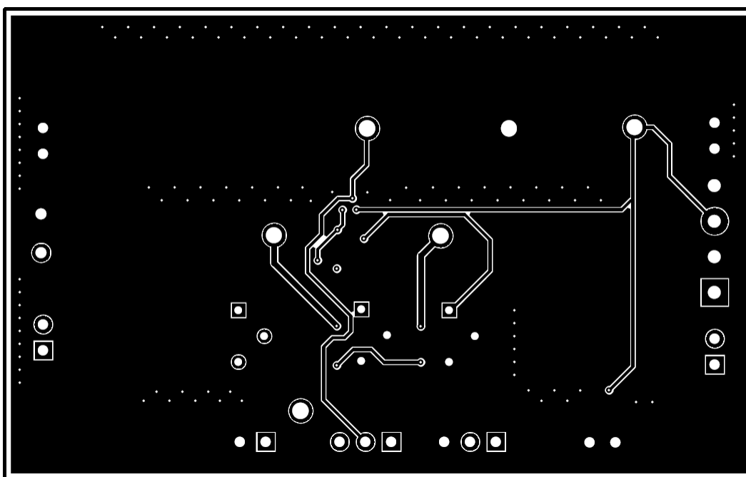
Figure 7. Bottom Layer
