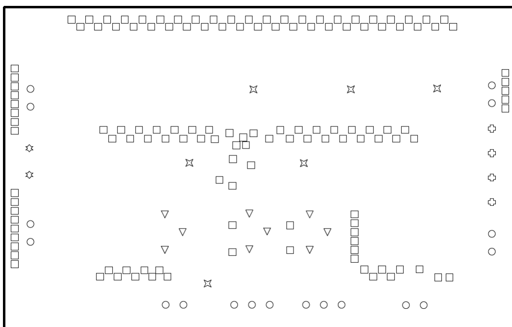
Figure 9. Drill Drawing
