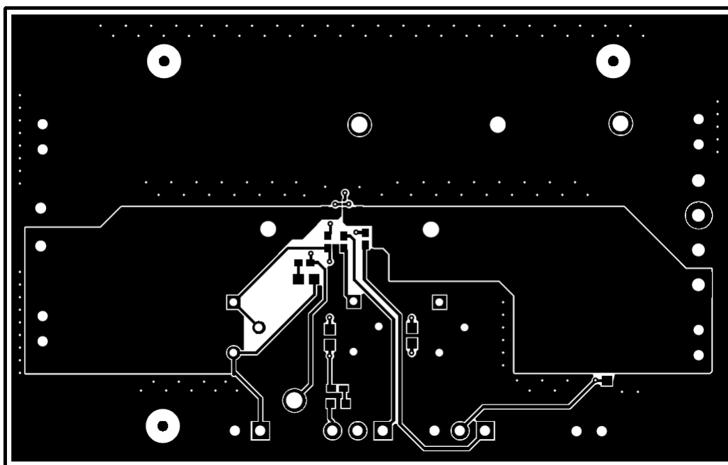
Figure 6. Top Layer
