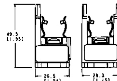
FIGURE 1 (ADDER)
