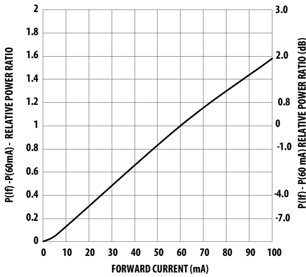
Figure 10: Normalized Typical Transmitter Output vs. Forward Current
